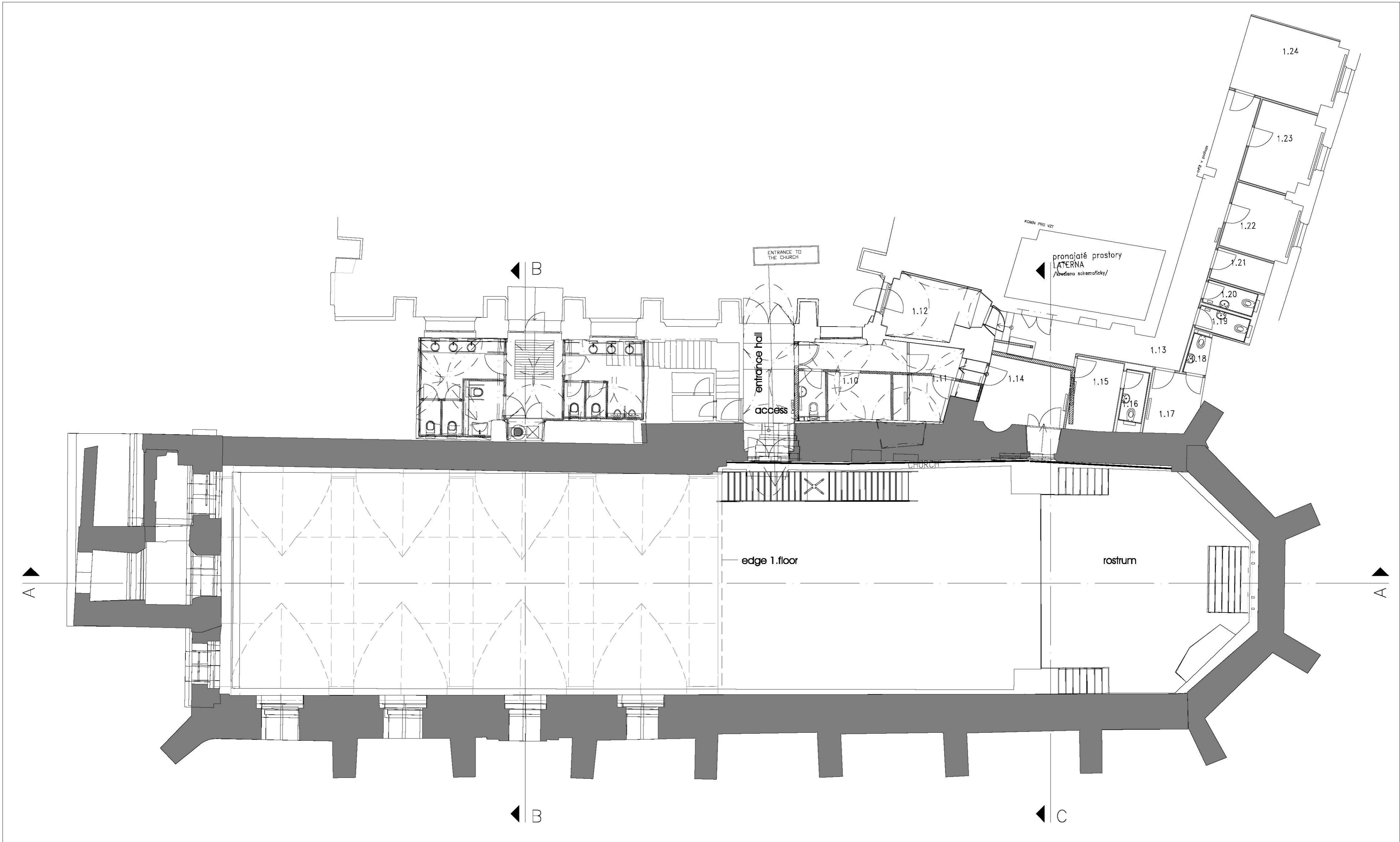
St. Anna Prague ground floor level
